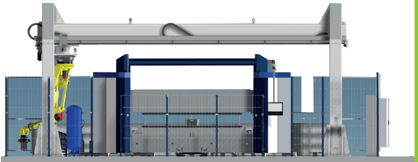
Schröder automation system with robot loading system and integrated MAK 4 Evolution UD folding machine.
